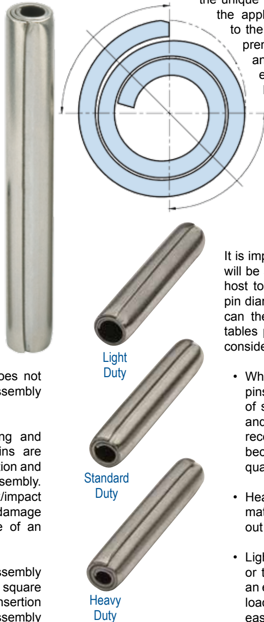
SPIROL® Coiled Spring Pins are available in three “duties” to enable the designer to choose the optimum combination of strength, flexibility and diameter to suit different host materials and application requirements.
